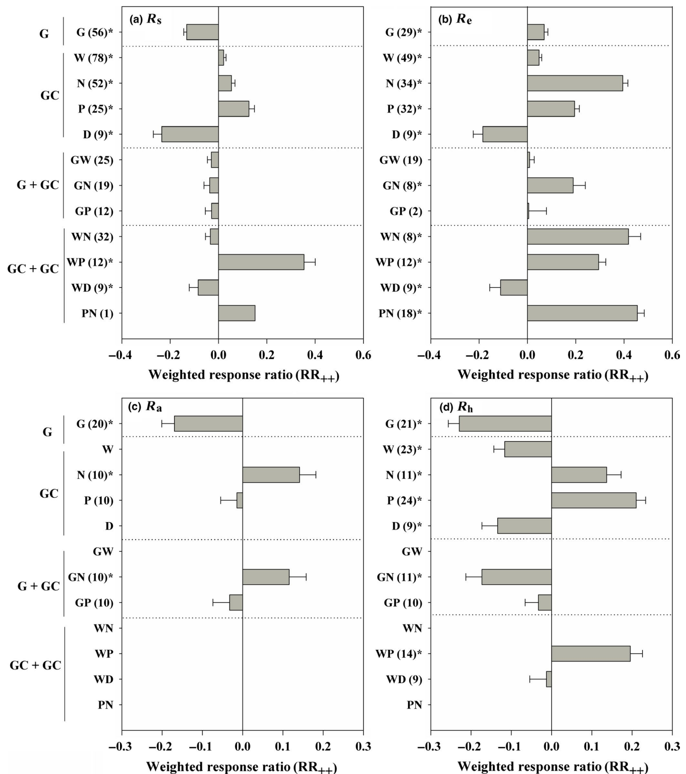
FIGURE 1 Weighted response ratio ( RR_{++} ) of soil respiration ( R_s , a), ecosystem respiration ( R_e , b), autotrophic respiration ( R_a , c) and heterotrophic respiration ( R_h , d) to the effects of single factor and two combined factors. Bars represent 95% confidence intervals. The vertical line was drawn at RR_{++} = 0 . G, W, N, P and D represent grazing, warming, nitrogen addition, increased precipitation and drought respectively. G, grazing; GC, all single-global climate change factor treatments; G + GC, grazing combined with a global climate change factor; GC + GC, two combined global climate change factors
